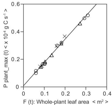
Figure 3: Light-saturated whole-plant photosynthetic rate on each day ( P_{\text{plant max}(t)} ) in relation to whole-plant leaf area on that day ( F_{(t)} ). Each series of symbols indicates one plant: circles, plant A ( n = 9 ); crosses, plant B ( n = 4 ); and triangles, plant C ( n = 5 ); P_{\text{plant max}(t)} was not obtained for the earliest days, in which only one to three leaves on the upper part of the stems were measured. Linear regression for each plant is significant ( r^2 > 0.995 , p < .01 for all plants). The line on the graph indicates regression through the entire data set ( r^2 > 0.993 , p < 1.0 \times 10^{-18} , n = 18 ), and its intercept is not significantly different from 0 ( p = .18 ): P_{\text{plant max}(t)} = 8.19 \times 10^{-7} + 1.69 \times 10^{-4} F_{(t)} .
